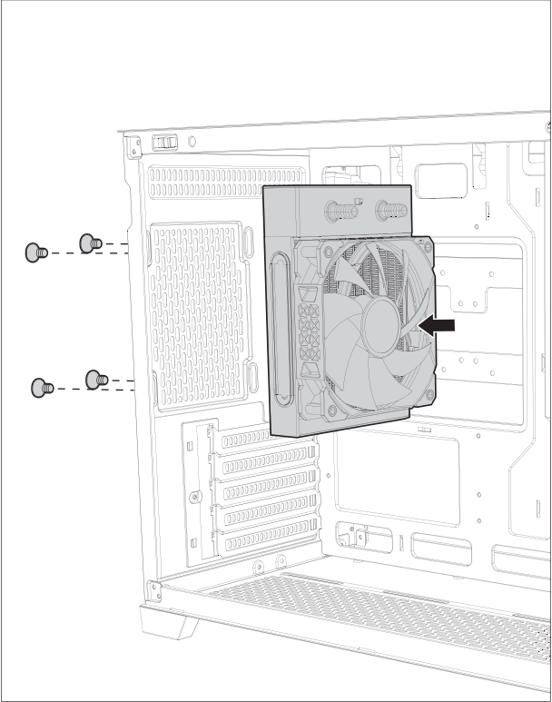
REAR RADIATOR
