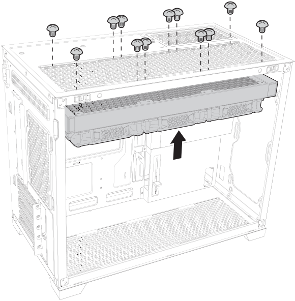
TOP RADIATOR
